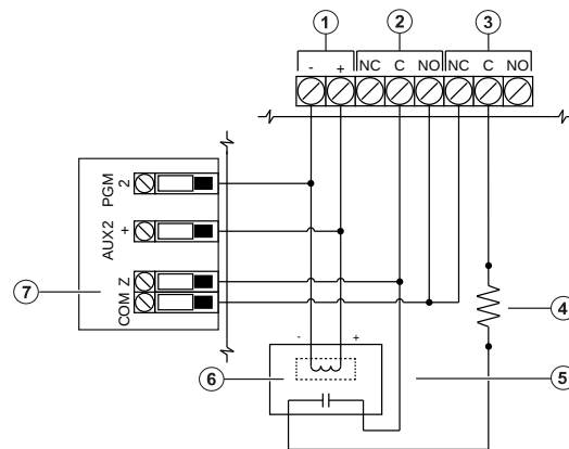
Figure 10: 4-wire smoke and heat detector wiring
