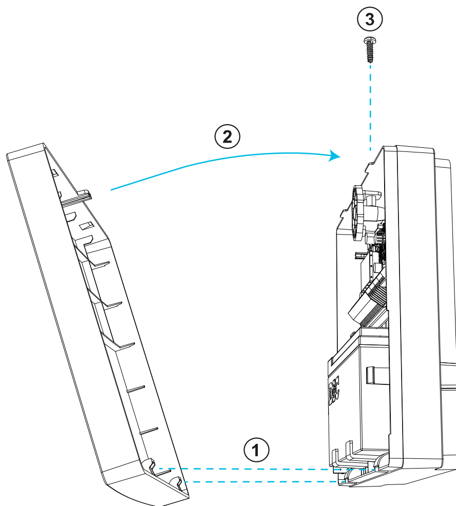
Figure 14: Attaching the cover
