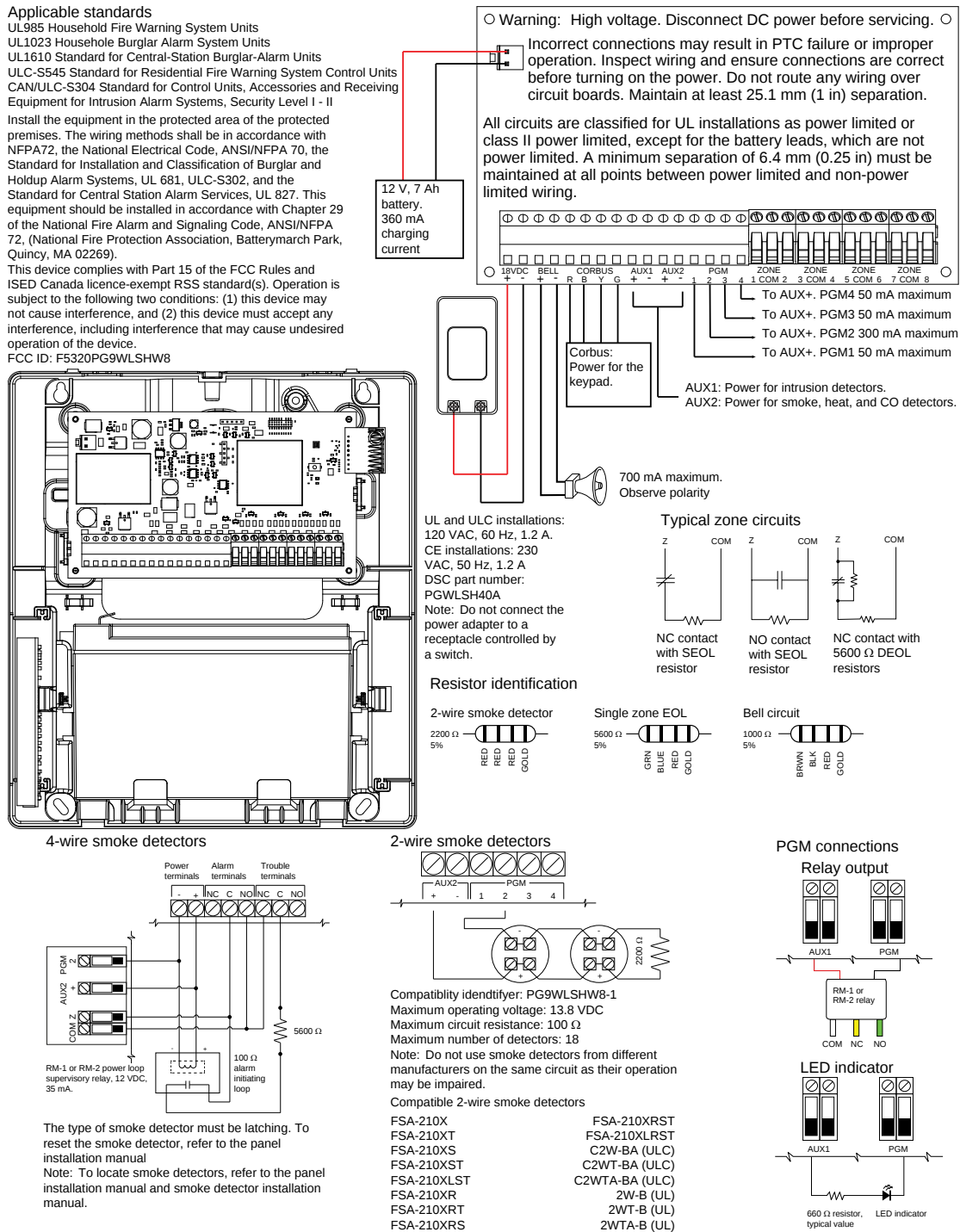
Figure 15: Wiring diagram
